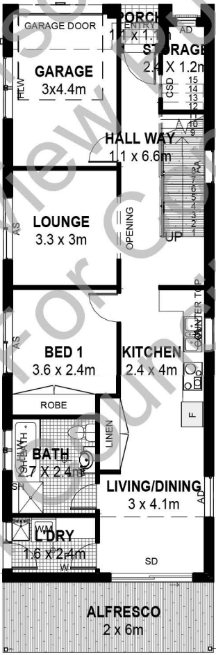
GROUND FLOOR PLAN 1 :150
